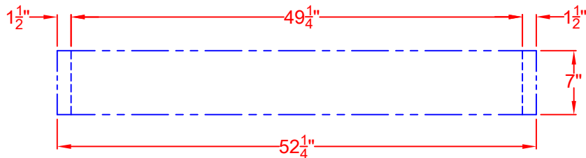
FRONT VIEW
