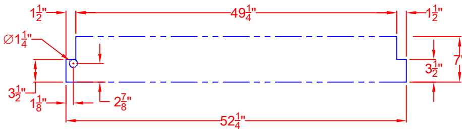
FRONT VIEW
