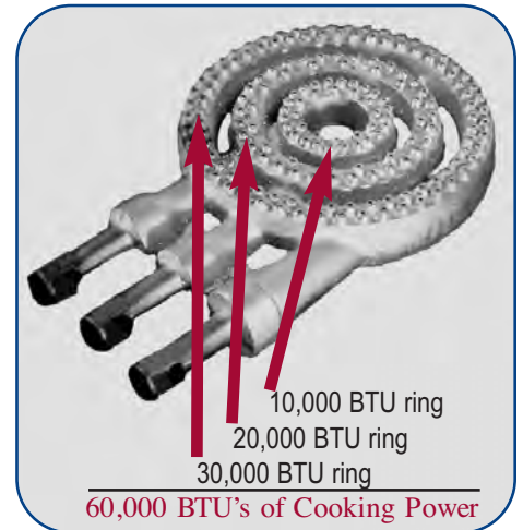
Triple Ring Single Burner Utility Stove
